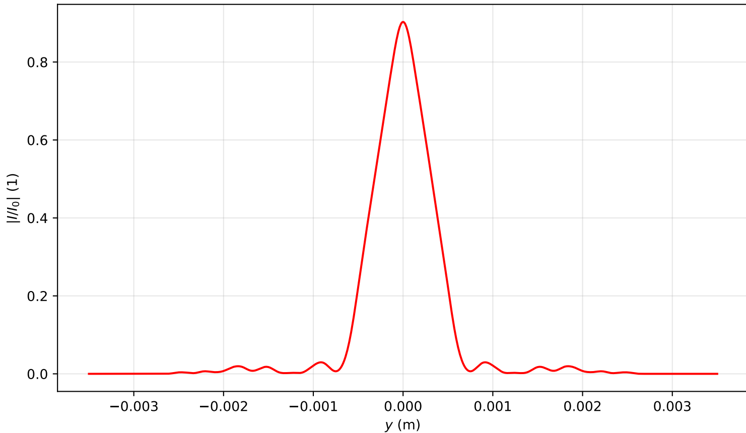
Intensity profile I(x=0, y, z=2.627)/I_0 , \text{Pin}=2.5\text{Pcr} , artificial time
